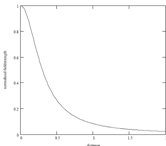
Figure 5. Typical behaviour of the magnetic field strength versus distance (example), for a transmitting antenna with a diameter of 0.8 m.
